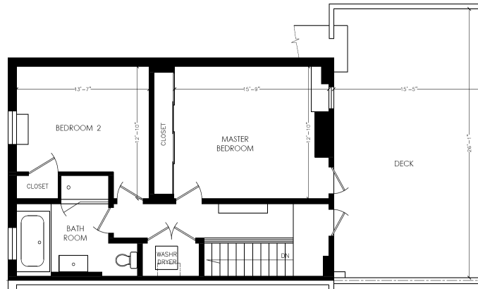
THIRD FLOOR FLOOR AREA 719 SQUARE FEET
