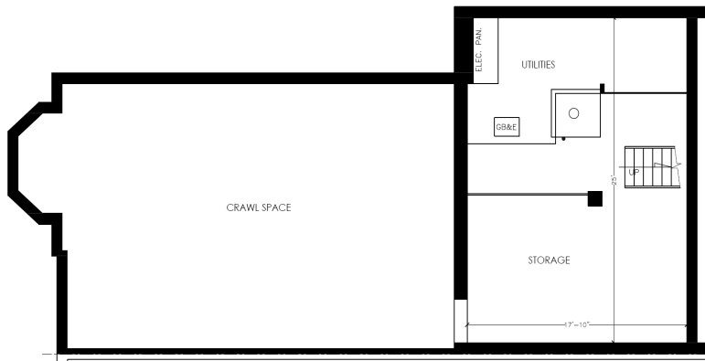
BASEMENT FLOOR AREA 526 SQUARE FEET
